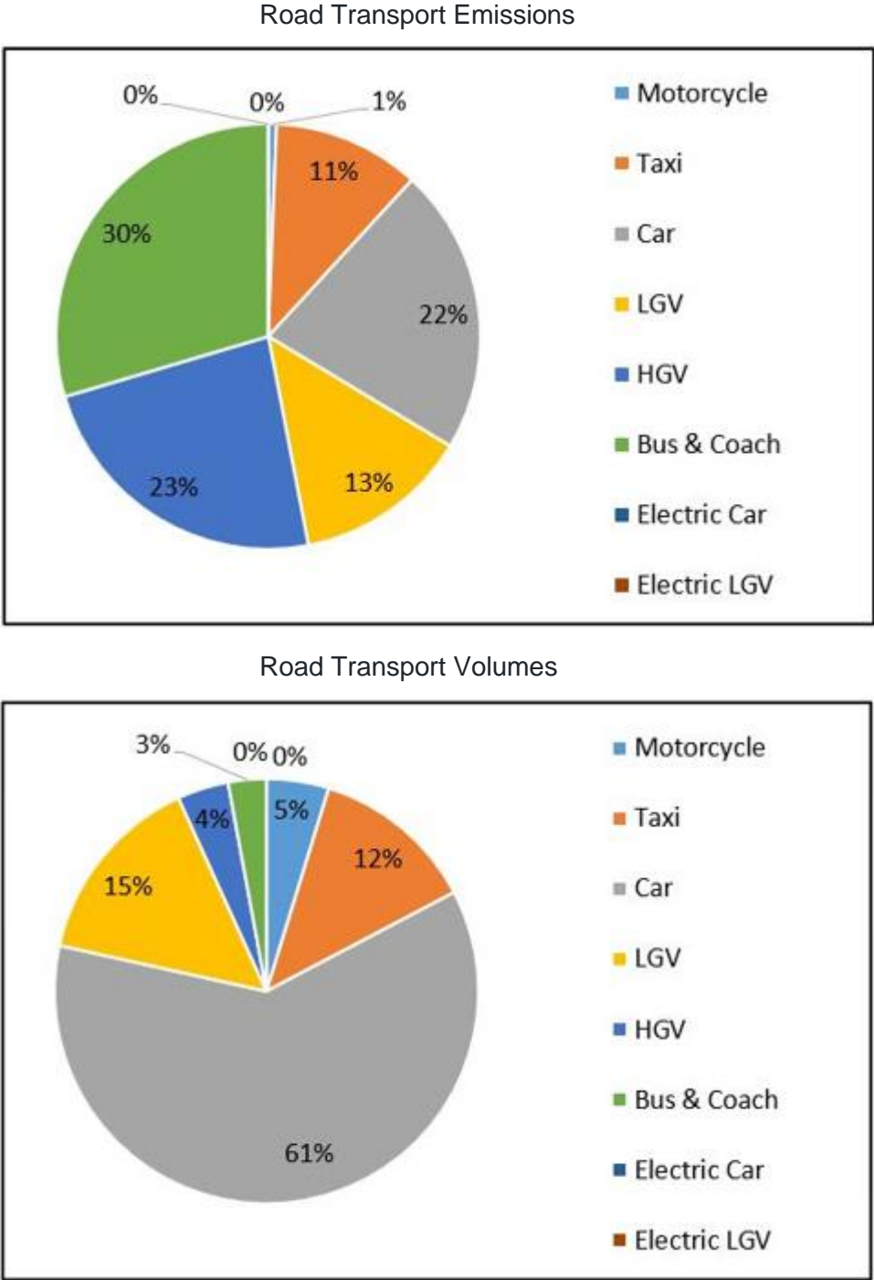
Figure 6 - Road Transport NO x Emissions and Volumes
