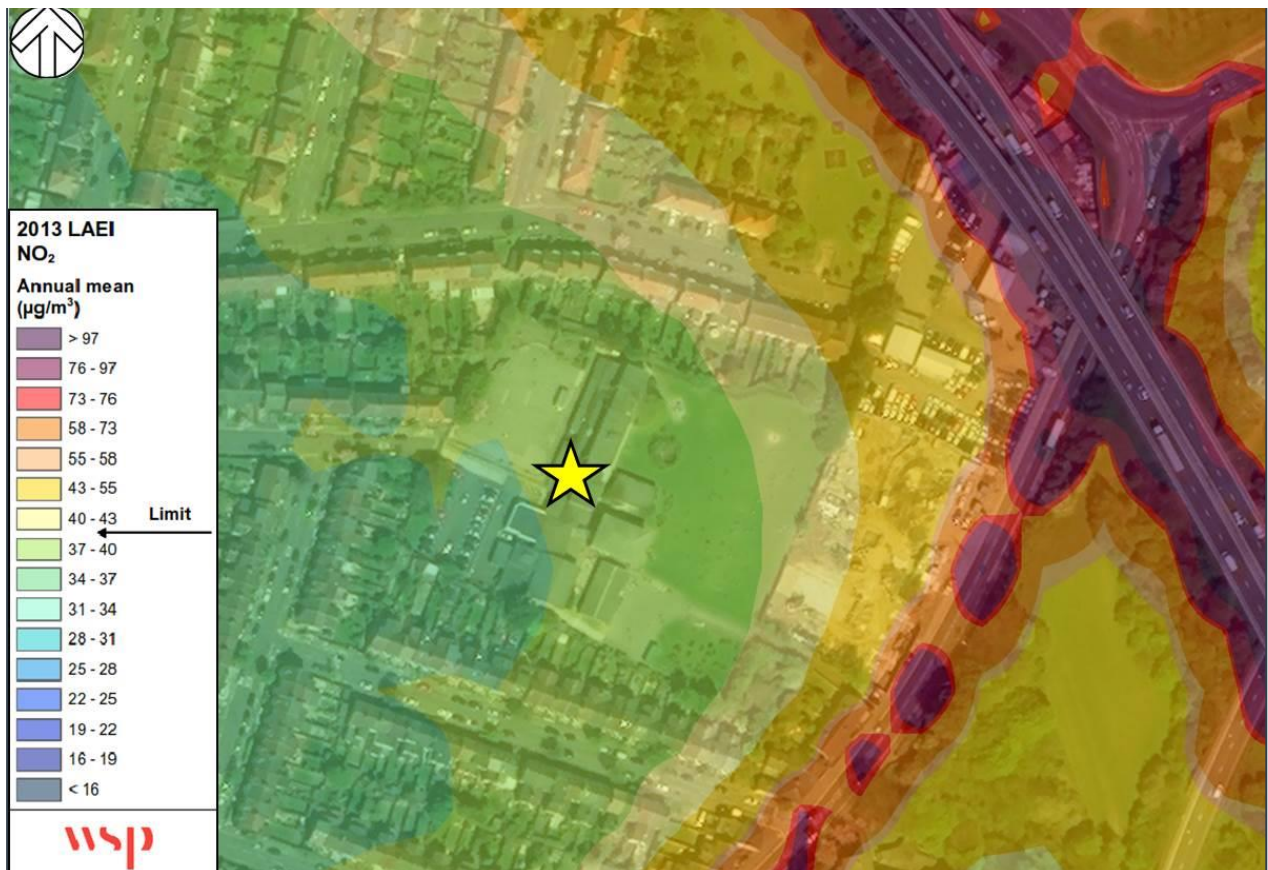
Figure 5 – Localised Air Quality modelling around Oakdale Junior School
